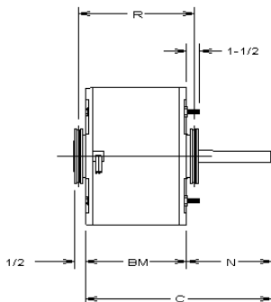
Adapter 621529-002 for Fleximount
